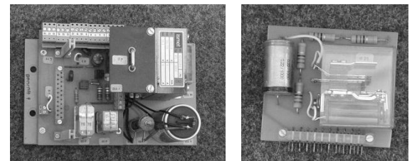
old Grid Keying Unit Chassis and Relay Plate
