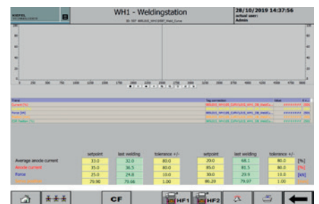
Welding curve
