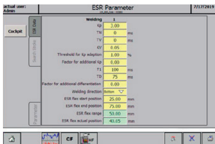
Regulation tuning
